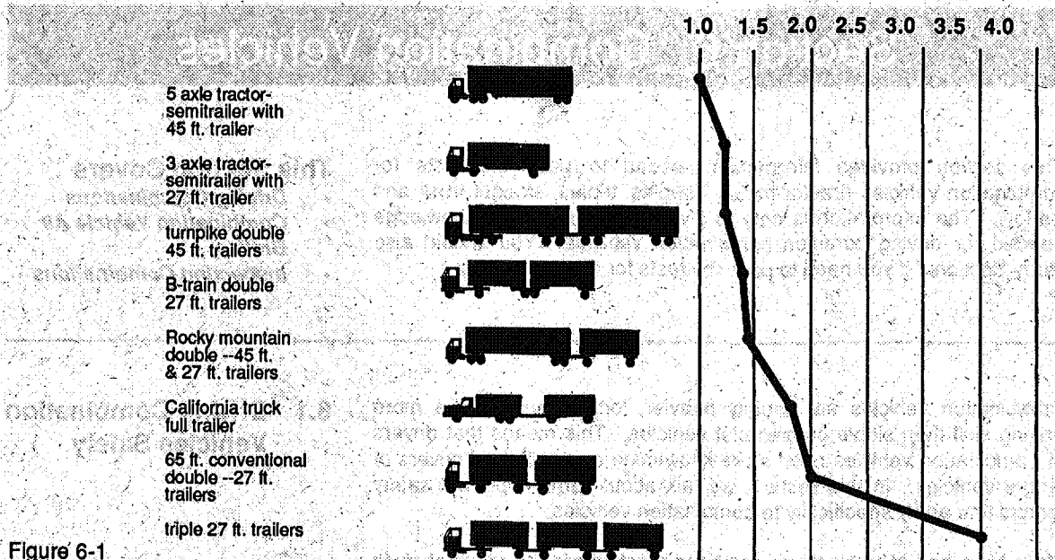
Influence of Combination Type on Rearward Amplification
