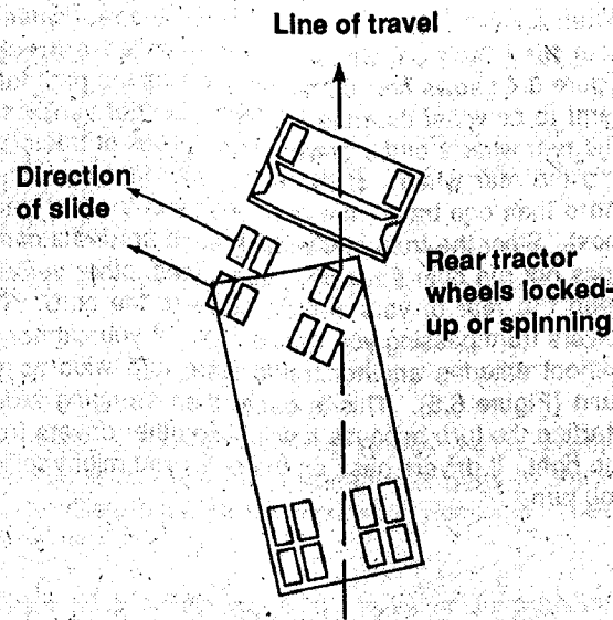
Figure 6-2 Tractor Jackknife
